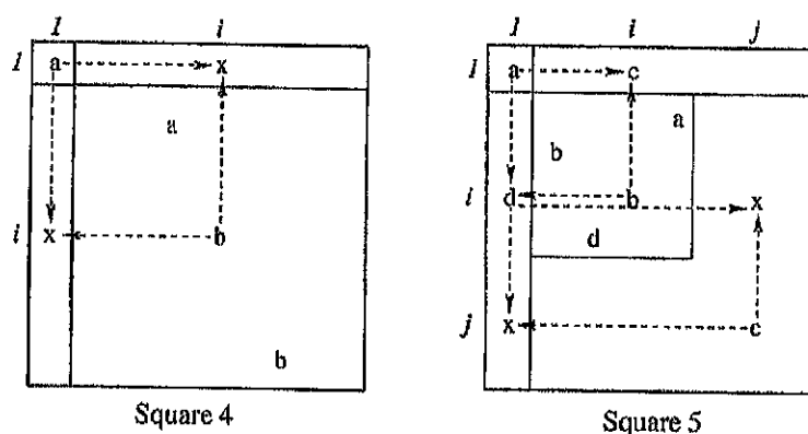
Fig. 3. Square 4: Illustration for the proof of Lemma 2. By applying # as shown, we find the first row contains only non-empty cells, a contradiction. Square 5: Illustration for the proof of Theorem 1. If an element c lies in the first row above the small square and also on the diagonal below and to the right of the small square, we find a non-empty cell x in the first column, below the small square, as shown.
