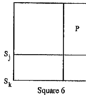
Fig. 4. The region P in the proof of Theorem 2.
