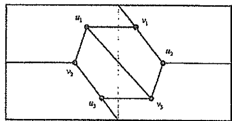
Embedding of K_{3,3} on S_1
