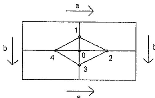
Embedding of K_5 on S_1
