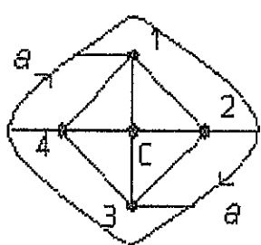
Embedding of K_5 on N_1 ( N_1 is also known as a projective plane.)
