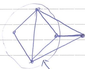
Induced subgraph
