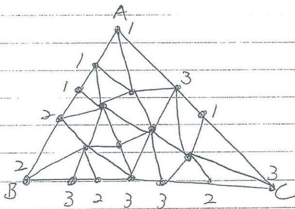
Figure 1, Triangulation of ABC
