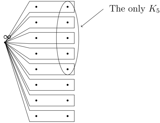
Figure for (2m+1, \{3, 5\}, 1) PBD
