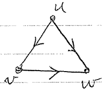
(Transitive)
