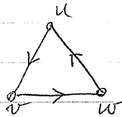
(Not transitive)
